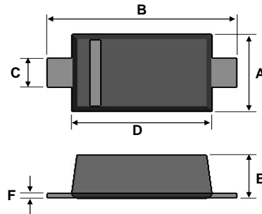
SOD-123F
